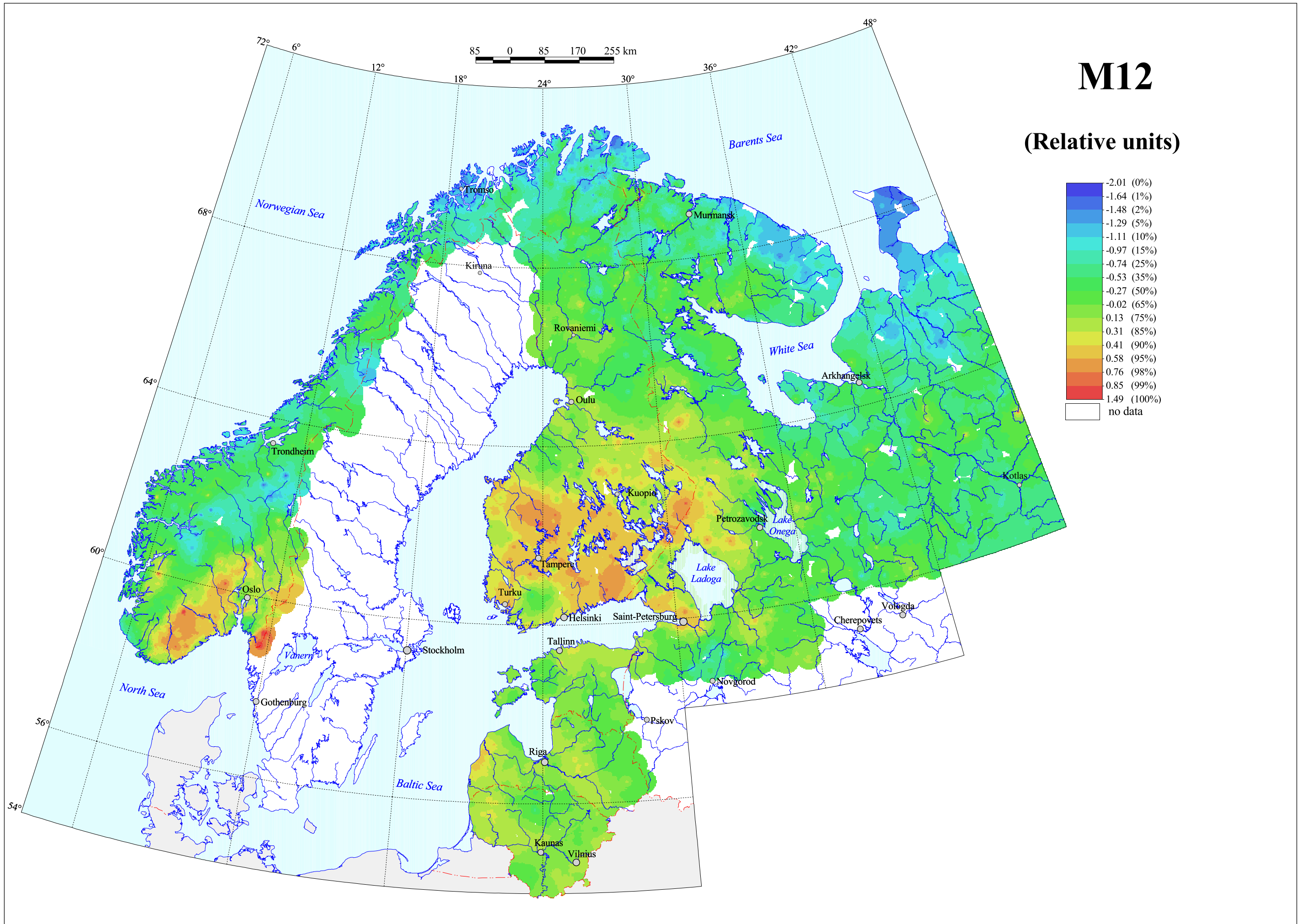
M12 (Rb, TI) in Terrestrial Moss, Total Content
